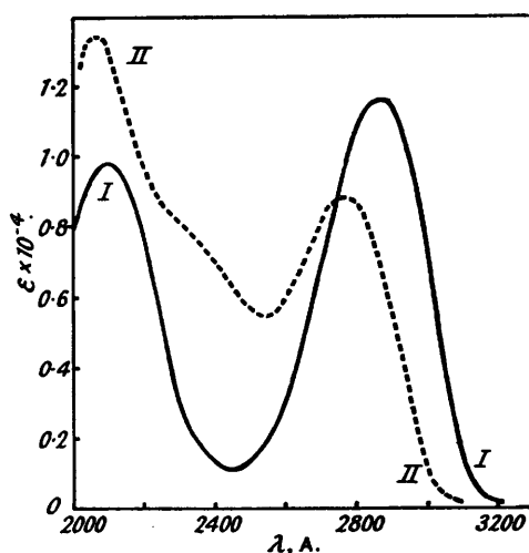
I. 5-Methylcytosine deoxyriboside in N/100\text{-HCl} . II. 5-Methylcytosine deoxyriboside in N/90\text{-NaOH} .
